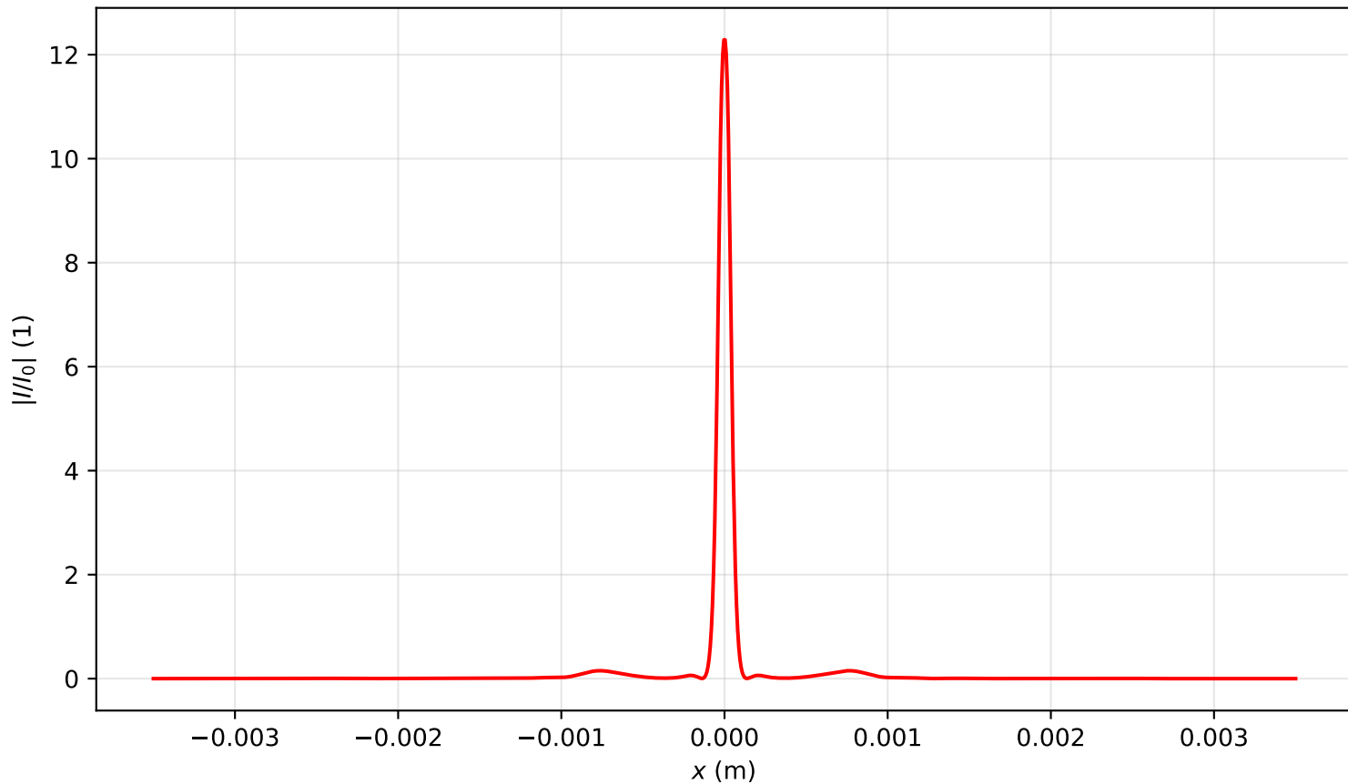
Intensity profile I(x, y = 0, z = 1.433)/I_0 , P_{in}=8.5P_{cr} , artificial time
